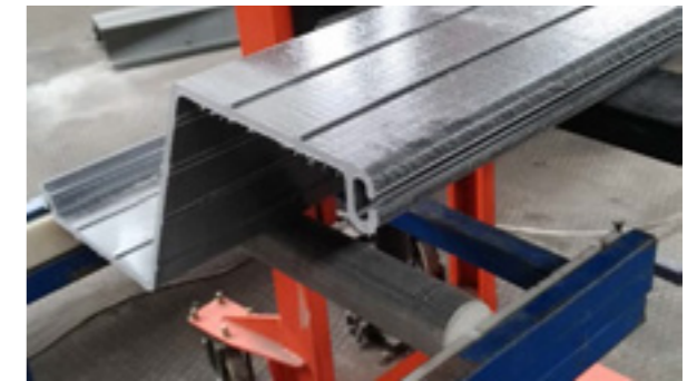
PVC SHEET PILE FOR SHORE PROTECTION
