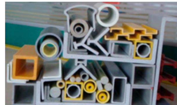
BALKS, CHANNELS AND OTHER BUILDING PROFILES
